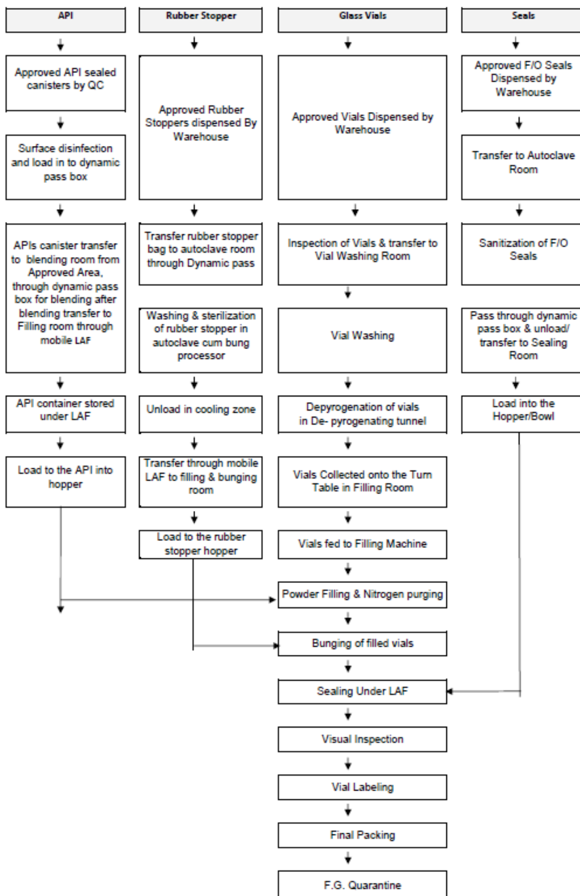
Process Flow chart for Dry Injection Blended Product (Blend of two drugs) Manufacturing
